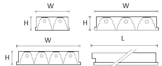
INSTALLATION RECESS T-BAR CEILING
